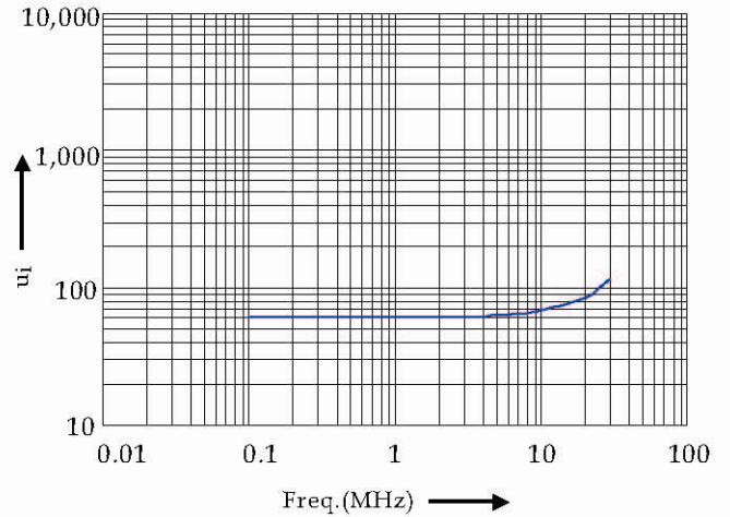
Initial permeability Frequency
