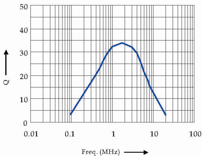
Quality factor vs Frequency
